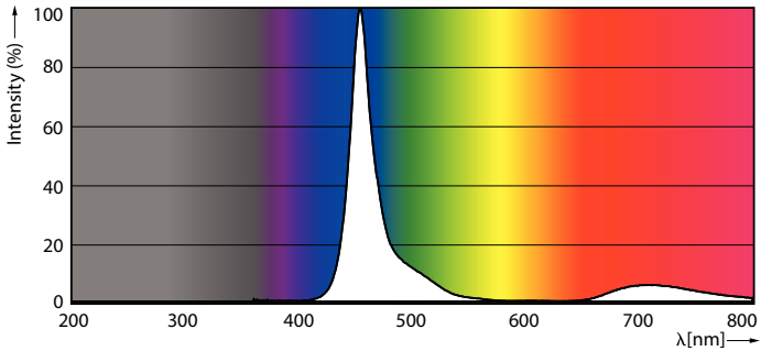
Spectral Power Distribution Colour - 8A19/LED/BLEU/P/ND 120V 4/1FB
