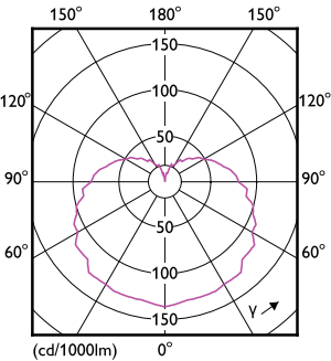
Light Distribution Diagram - 8A19/LED/BLEU/P/ND 120V 4/1FB
