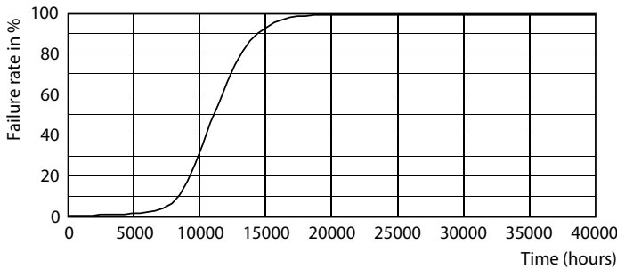
Life Expectancy Diagram - 8A19/LED/BUE/P/ND 120V 4/1FB
