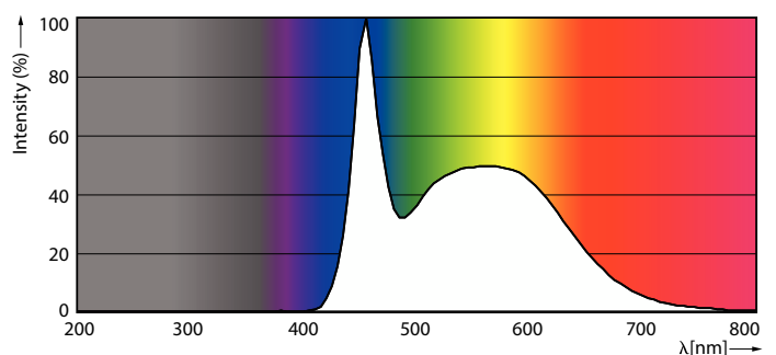
Spectral Power Distribution Colour - TForce Core HB 45-50W E40 865
