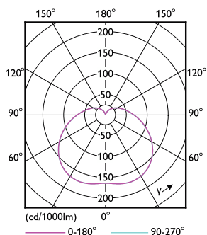
Light Distribution Diagram - TForce Core HB 45-50W E40 865
