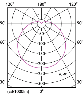
Light Distribution Diagram - ESS LEDBulb 19W E27 6500K HV 1PF/20 AR
