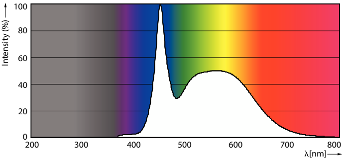
Spectral Power Distribution Colour - ESS LEDBulb 19W E27 6500K HV 1PF/20 AR
