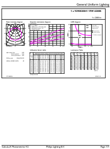
General uniform lighting - ESS LEDBulb 19W E27 6500K HV 1PF/20 AR
