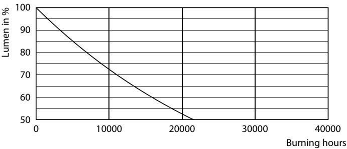
Lumen Maintenance Diagram - ESS LEDBulb 19W E27 6500K HV 1PF/20 AR
