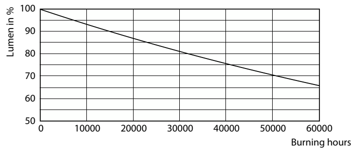
Lumen Maintenance Diagram - TForce LED Road 90-55W E40 740
