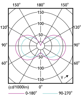
Light Distribution Diagram - CLA LEDBulb DT9-60W E27 CRI90 G93 CL
