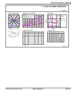
General uniform lighting - MAS LEDtube VLE 1500mm UO 24W 830 T8
