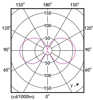
Light Distribution Diagram - CLA LEDBulb ND 8.5-75W A60 E27 827 CL
