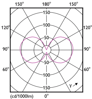
Light Distribution Diagram - CLA LEDLuster ND 6.5-60W P45 E27 827 CL
