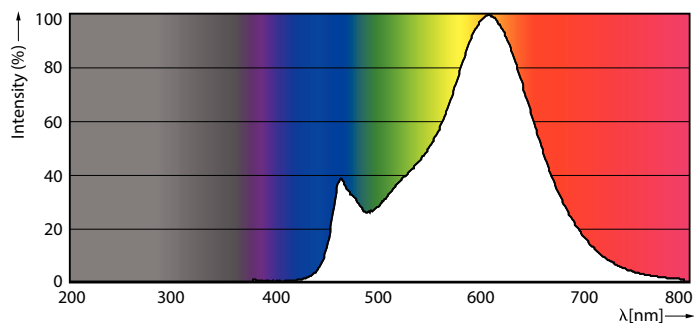
Spectral Power Distribution Colour - CLA LEDLuster ND 6.5-60W P45 E27 827 CL
