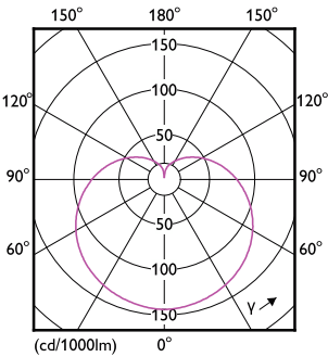
Light Distribution Diagram – CorePro LEDbulb ND 19-150WA67E27 827FR
