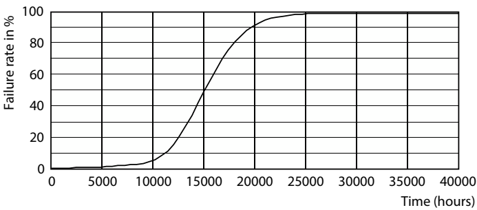
Life Expectancy Diagram - CorePro LEDbulb ND 17.5-150WA67E27 840FR
