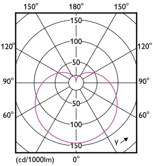
Light Distribution Diagram - CorePro LEDbulb ND 17.5-150WA67E27 840FR
