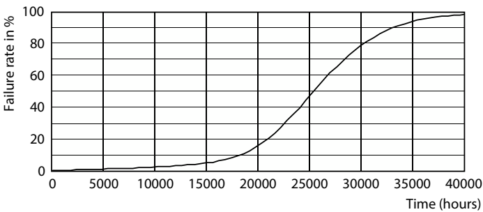
Life Expectancy Diagram - MAS LEDspotLV D 20-100W 940 AR111 24D
