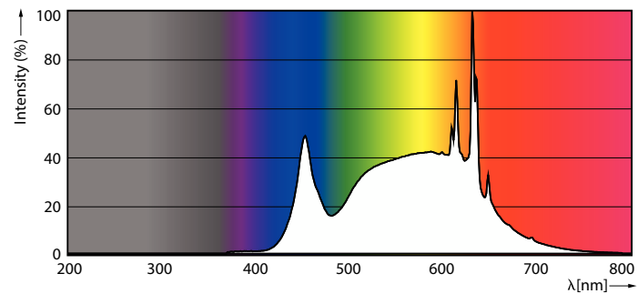
Spectral Power Distribution Colour - MAS LEDspotLV D 20-100W 940 AR111 24D
