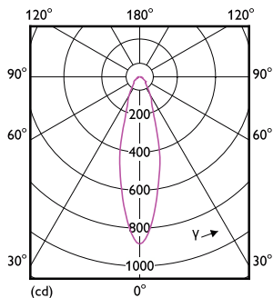
Light Distribution Diagram - MAS LEDspotLV D 20-100W 940 AR111 24D
