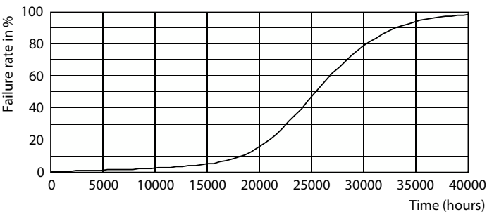
Life Expectancy Diagram - MAS LEDspotLV D 20-100W 940 AR111 24D
