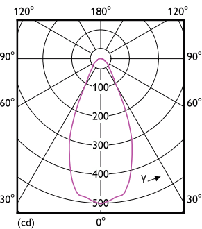
Light Distribution Diagram - MAS LEDspotLV D 20-100W 940 AR111 45D
