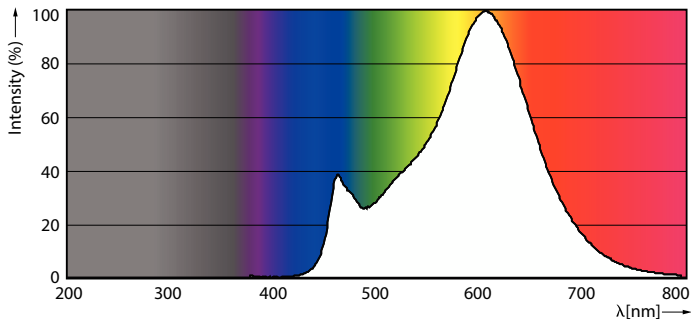
Spectral Power Distribution Colour - CLA LEDBulb ND 17-150W A67 E27 827 CL
