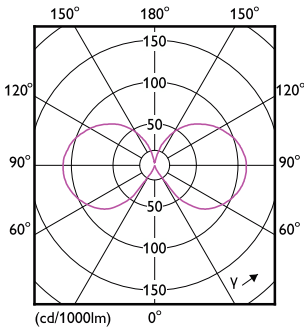
Light Distribution Diagram - CLA LEDBulb ND 17-150W A67 E27 827 CL
