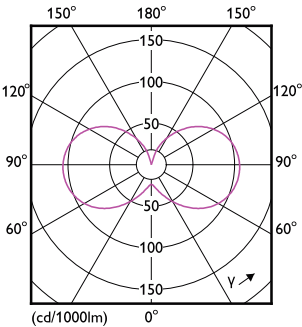
Light Distribution Diagram - CorePro LEDcapsule ND 4.8-60W G9 830
