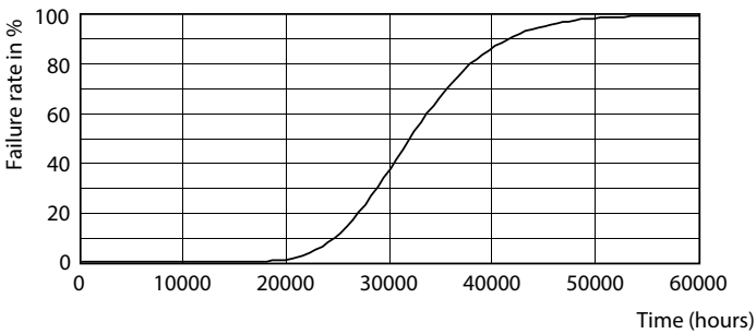
Life Expectancy Diagram - CorePro LED Circular 20W 840 G10q
