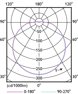
Light Distribution Diagram - CorePro LED Circular 20W 865 G10q
