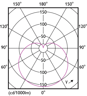
Light Distribution Diagram - CorePro LEDbulb D 10.5-75W A60 E27 927
