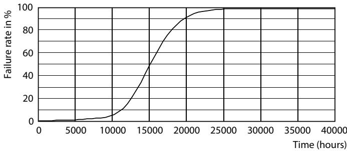
Life Expectancy Diagram - CorePro LEDbulb D 13-100W A60 E27 927
