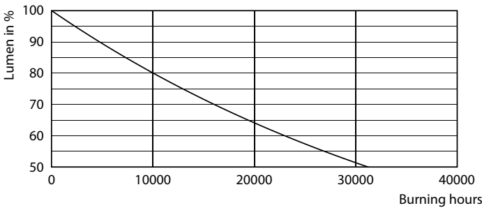
Lumen Maintenance Diagram - CorePro LEDbulb D 13-100W A60 E27 927
