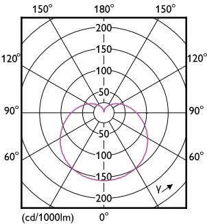
Light Distribution Diagram - CorePro LEDbulb D 13-100W A60 E27 927
