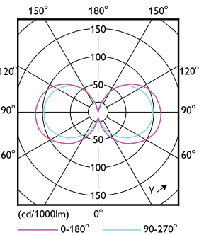
Light Distribution Diagram - 5.5G16.5/PER/927-922/CL/G/E26/WGX 1FBT20
