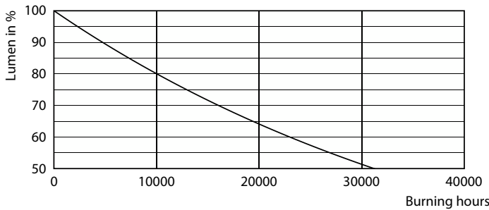
Lumen Maintenance Diagram - 5.5G16.5/PER/927-922/CL/G/E26/WGX 1FBT20
