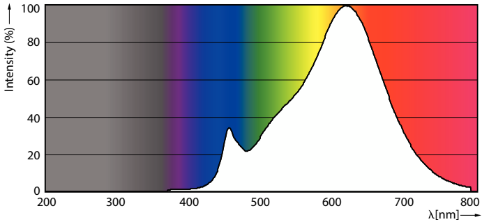
Spectral Power Distribution Colour - 5.5G16.5/PER/927-922/CL/G/E26/WGX 1FBT20
