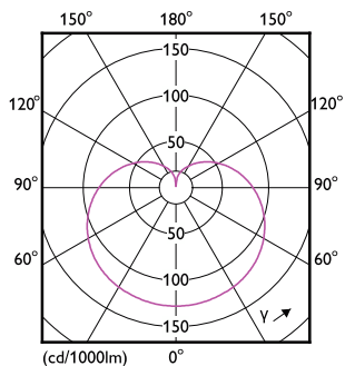
Light Distribution Diagram - MASLEDbulb DT 14-100WE27 927-922 A67FR
