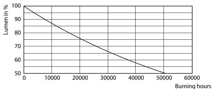
Lumen Maintenance Diagram - MASLEDbulb DT 14-100WE27 927-922 A67FR
