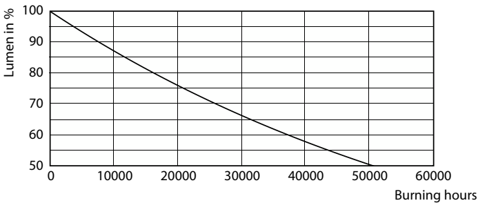
Lumen Maintenance Diagram - MASLEDbulb DT 14-100WE27 927-922 A67FR
