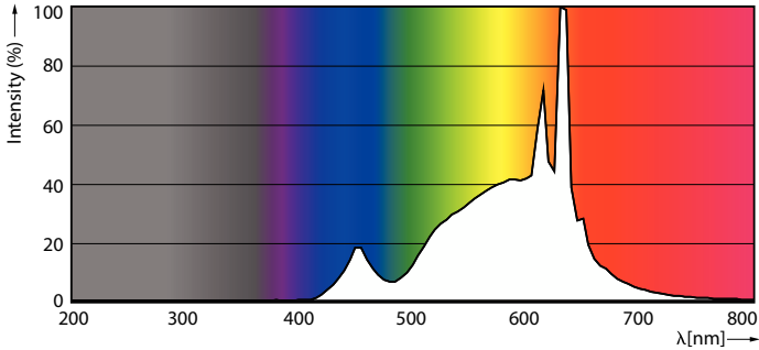
Spectral Power Distribution Colour - MASLEDbulb DT 14-100WE27 927-922 A67FR
