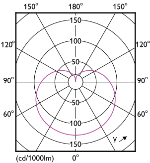
Light Distribution Diagram - MASLEDbulb DT 14-100WE27 927-922 A67FR
