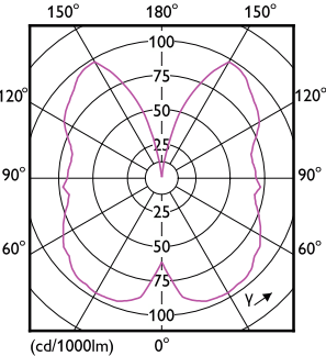
Light Distribution Diagram - CLA LEDBulb D 5.5-25W T32 E27 GOLD SP CL
