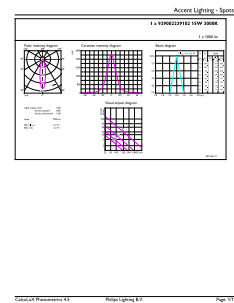
General uniform lighting - MAS LED ExpertColor 15-75W 930 AR111 24D
