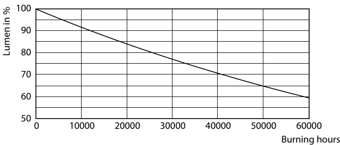
Lumen Maintenance Diagram - MAS LED ExpertColor 15-75W 927 AR111 40D
