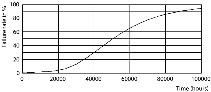
Life Expectancy Diagram - 27CC/LED/840/ND E26 BB 12/1
