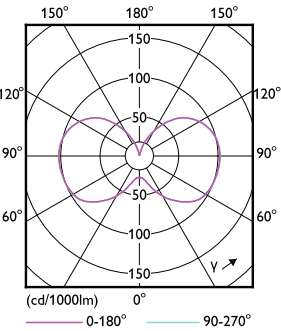
Light Distribution Diagram - 27CC/LED/850/ND E26 BB 6/1
