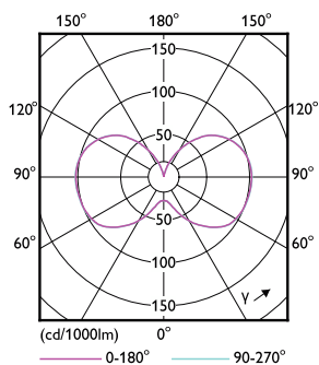
Light Distribution Diagram - 27CC/LED/830/ND EX39 BB 6/1
