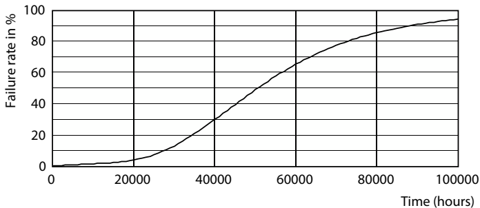
Life Expectancy Diagram - 27CC/LED/830/ND EX39 BB 6/1
