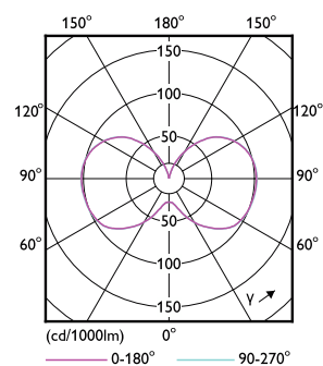
Light Distribution Diagram - 27CC/LED/840/ND EX39 BB 6/1
