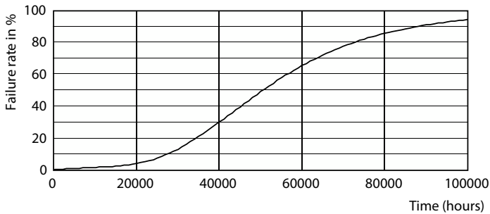
Life Expectancy Diagram - 36CC/LED/840/ND E26 BB 12/1
