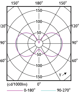
Light Distribution Diagram - 36CC/LED/840/ND E26 BB 6/1
