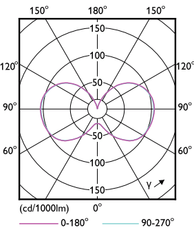
Light Distribution Diagram - 36CC/LED/840/ND EX39 BB 6/1
