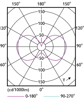
Light Distribution Diagram - 36CC/LED/850/ND EX39 BB 12/1
