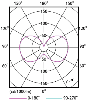
Light Distribution Diagram - 54CC/LED/830/ND EX39 BB 12/1
