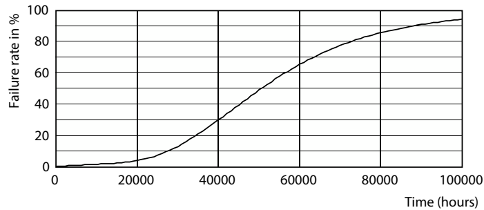
Life Expectancy Diagram - 54CC/LED/830/ND EX39 BB 12/1
