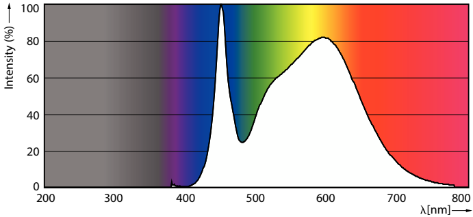
Spectral Power Distribution Colour - 54CC/LED/840/ND EX39 BB 12/1
