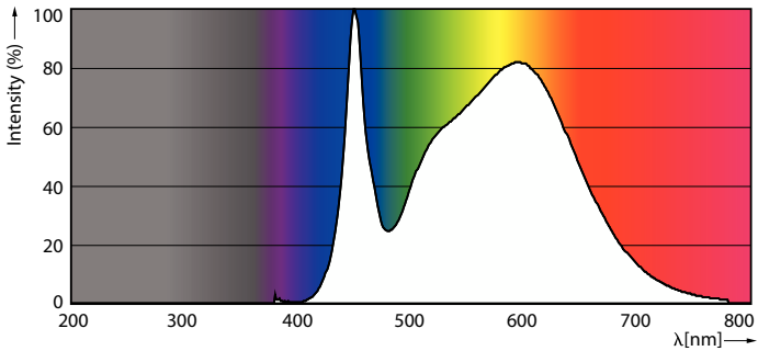
Spectral Power Distribution Colour - 54CC/LED/840/ND EX39 BB 6/1
