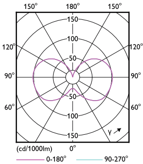
Light Distribution Diagram - 54CC/LED/840/ND EX39 BB 6/1
