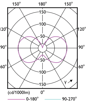
Light Distribution Diagram - 54CC/LED/850/ND EX39 BB 6/1
