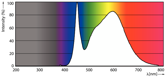
Spectral Power Distribution Colour - 63CC/LED/840/ND EX39 BB 12/1
