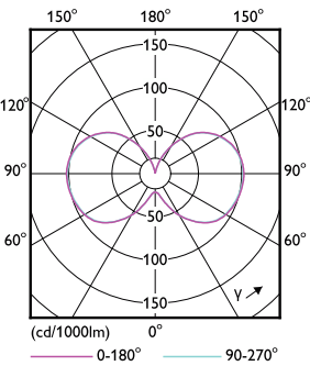
Light Distribution Diagram - 63CC/LED/840/ND EX39 BB 6/1
