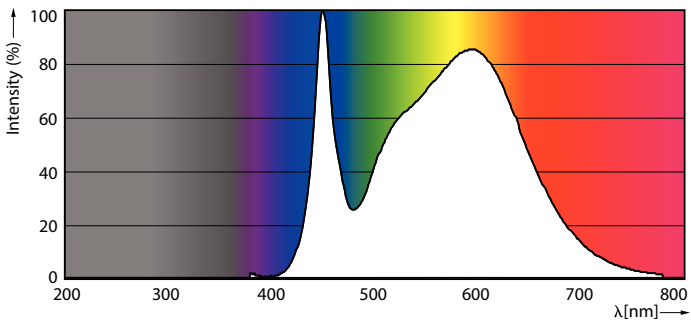
Spectral Power Distribution Colour - 63CC/LED/840/ND EX39 BB 6/1
