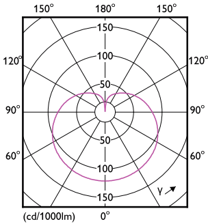
Light Distribution Diagram - 14A21/LED/927/P/E26/3WAY ND 4/1FB T20
