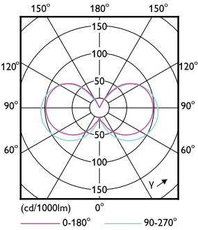
Light Distribution Diagram - 8ST19/PER/927-922/CL/G/E26/WGX PF T20
