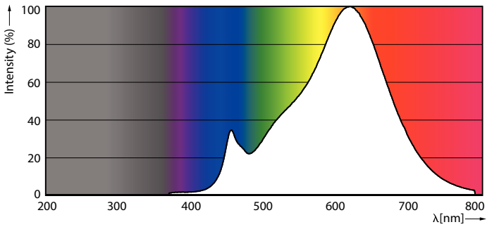
Spectral Power Distribution Colour - 8ST19/PER/927-922/CL/G/E26/WGX PF T20
