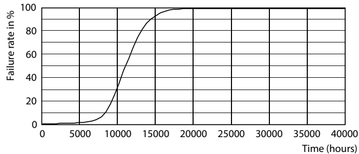
Life Expectancy Diagram - CorePro LEDcapsule 2-25W ND G9 827 G
