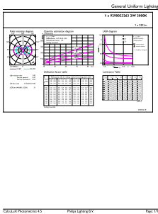
General uniform lighting - CorePro LEDcapsule 2-25W ND G9 830 G
