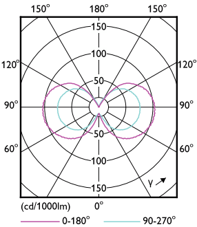
Light Distribution Diagram - CorePro LEDcapsule 2-25W ND G9 830 G
