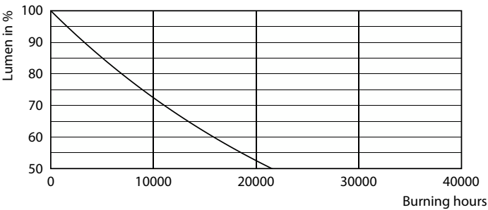
Lumen Maintenance Diagram - CorePro LEDcapsule 3.5-40W ND G9 827 G
