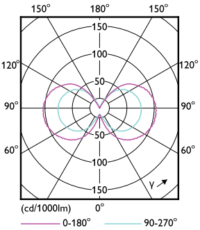
Light Distribution Diagram - CorePro LEDcapsule 3.5-40W ND G9 827 G
