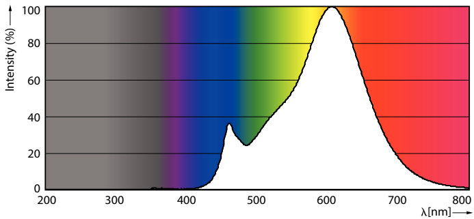
Spectral Power Distribution Colour - CorePro LEDcapsule 3.5-40W ND G9 827 G
