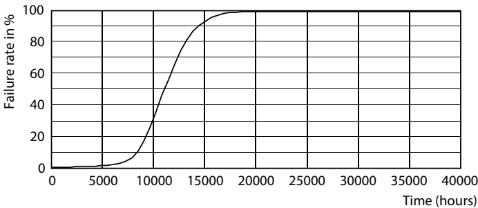
Life Expectancy Diagram - CorePro LEDcapsule 3.5-40W ND G9 827 G
