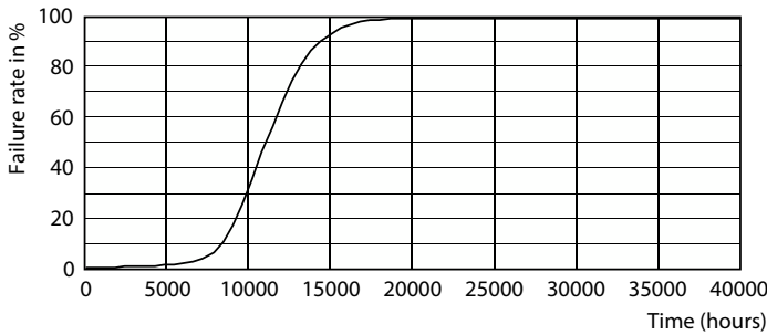
Life Expectancy Diagram - CorePro LEDcapsule 3.5-40W ND G9 830 G
