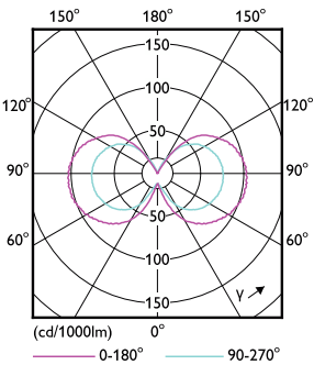
Light Distribution Diagram - CorePro LEDcapsule 3.5-40W ND G9 830 G
