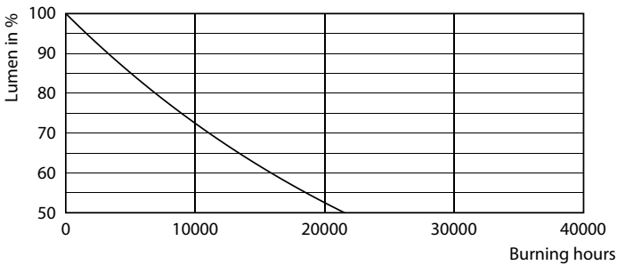
Lumen Maintenance Diagram - CorePro LEDcapsule 3.5-40W ND G9 830 G
