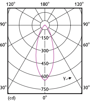
Light Distribution Diagram - MAS LEDspot VLE D 5-50W GU10 830 36D 5CT
