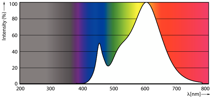
Spectral Power Distribution Colour - MAS LEDspot VLE D 5-50W GU10 830 36D 5CT
