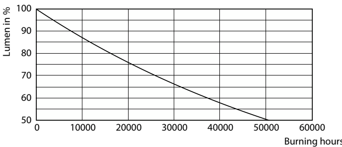
Lumen Maintenance Diagram - MAS LEDspot VLE D 5-50W GU10 830 36D 5CT
