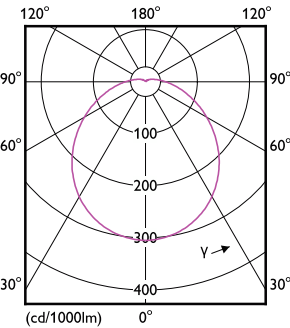
Light Distribution Diagram - 15BR30/PER/927-22/E26/WG/HO 4/1FB T20
