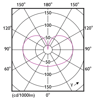
Light Distribution Diagram - LED classic 120W A67 E27 WW CL ND SRT4
