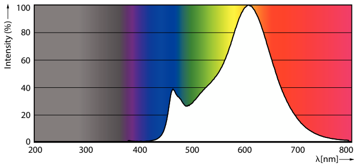
Spectral Power Distribution Colour - LED classic 120W A67 E27 WW CL ND SRT4
