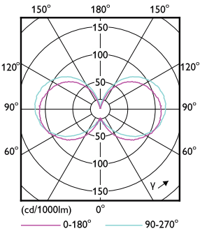
Light Distribution Diagram - CLA LEDBulb D 7.2-60W A60 E27 827 CL
