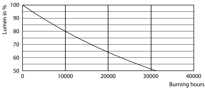
Lumen Maintenance Diagram - CLA LEDBulb DT12-100W E27 CRI90 A60 FR
