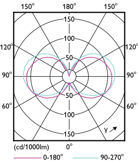
Light Distribution Diagram - CLA LEDBulb DT12-100W E27 CRI90 A60 FR
