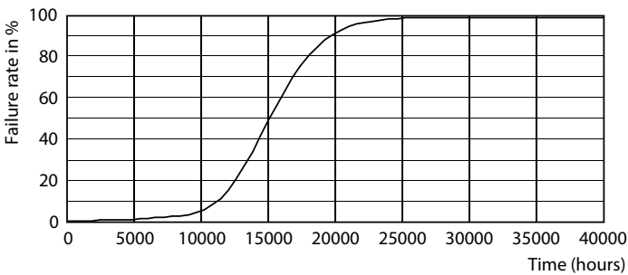
Life Expectancy Diagram - CLA LEDBulb DT12-100W E27 CRI90 A60 FR
